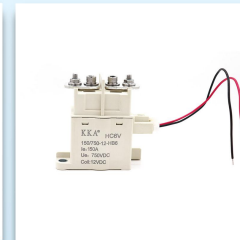
KKA-HC6V-150-750 Relay
